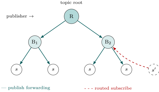
Fig. 3. Axon-tree formation. A new subscriber s' issues a routed subscribe toward \text{topicId} (red dashed); the first live axon role on the path (here, B_2 ) intercepts and adopts it. Publishes flow from the root R through the branches to all subscribers (teal solid). Tree healing under churn is the same mechanism: a subscriber whose parent dies re-issues its subscribe, attaches to whichever live ancestor is now closest, and continues receiving publishes after one refresh interval.
